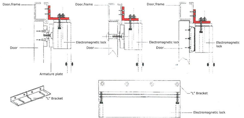
Example showing outward opening door
