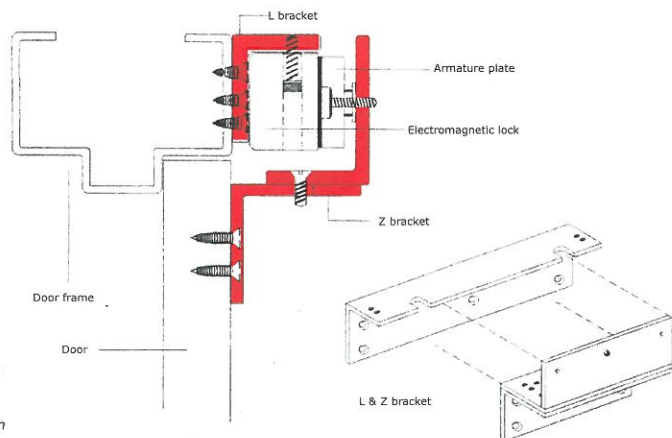
Example showing inward opening door
