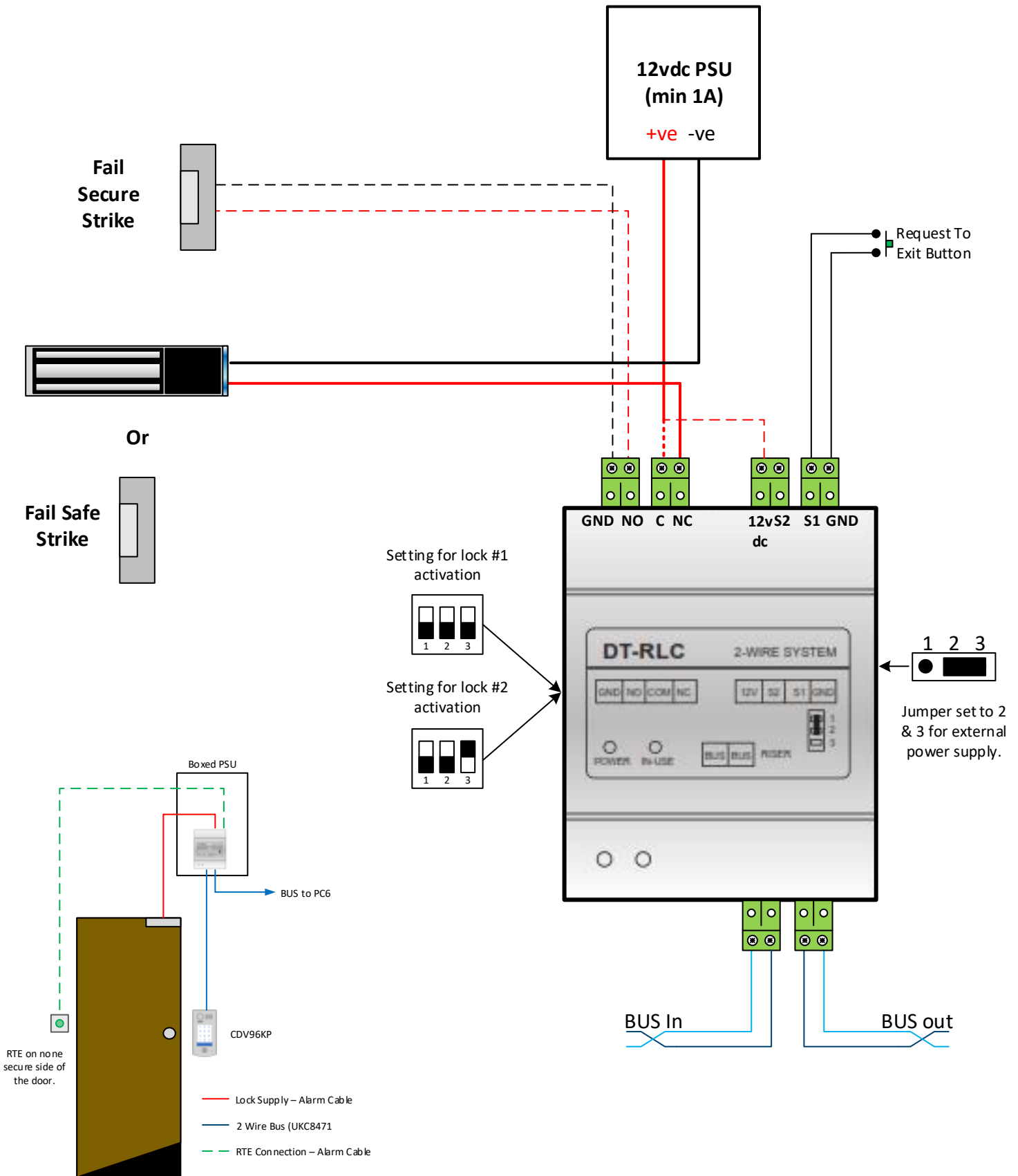
Wiring Layout Example
